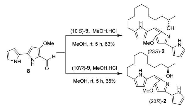
Scheme 4. Synthesis of ( S )- and ( R )-23-Hydroxyundecylprodiginines ((23 S )-2 and (23 R )-2)
